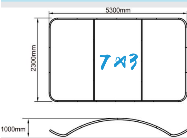
Frame 7x3
