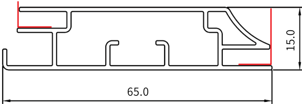
2.6 " /65mm Profile
