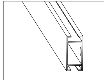
Stabilizer 44 TF-S2440
